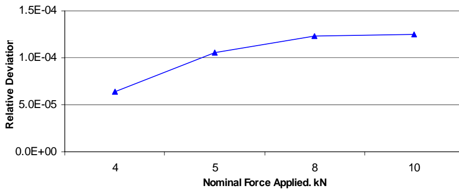
Graph 2. Maximum deviations for the force transducer F44076.
