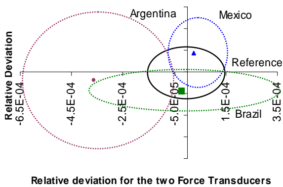
Graph 7. Youden Plot for 4 kN.
