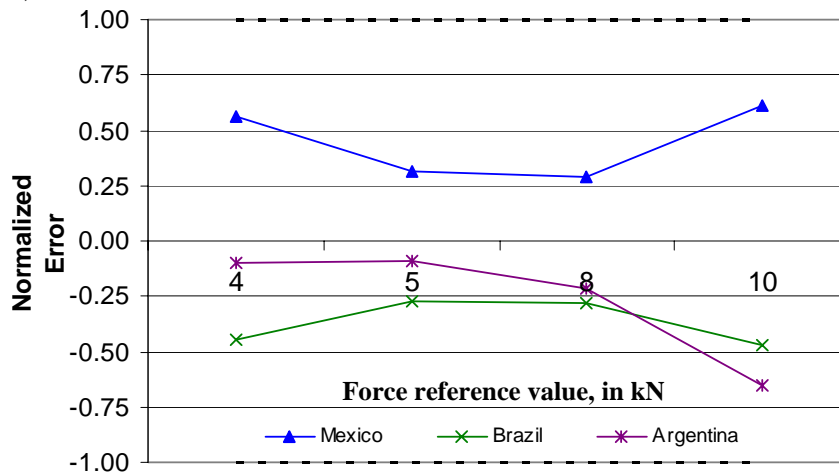
Graph 6. Normalized error (using standard uncertainty, k=1 ) for the force transducer F44076.
