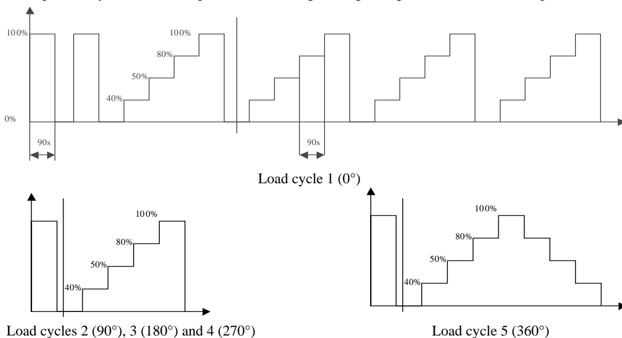
Figure 1. Comparison Load Cycles.
