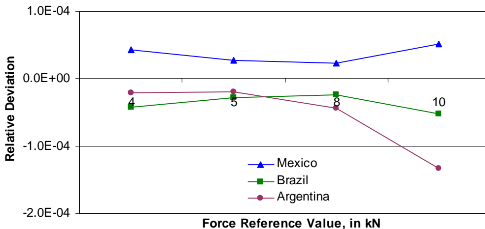
Graph 4. Relative deviation to the reference value of force with the force transducer F44076.
