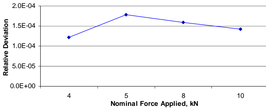
Graph 1. Maximum deviations for the force transducer G51316.
