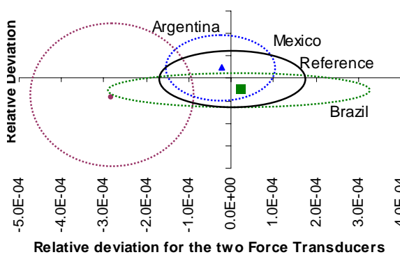
Graph 9. Youden Plot for 8 kN.
