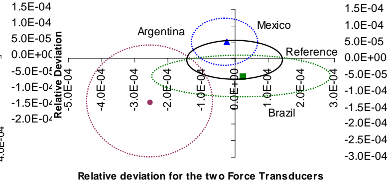
Graph 10. Youden Plot for 10 kN.
