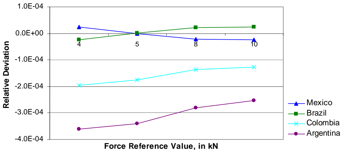
Graph 3. Relative deviation to the reference value of force with the force transducer G51316.
