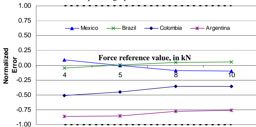
Graph 5. Normalized error (using standard uncertainty, k=1 ) for the force transducer G51316.
