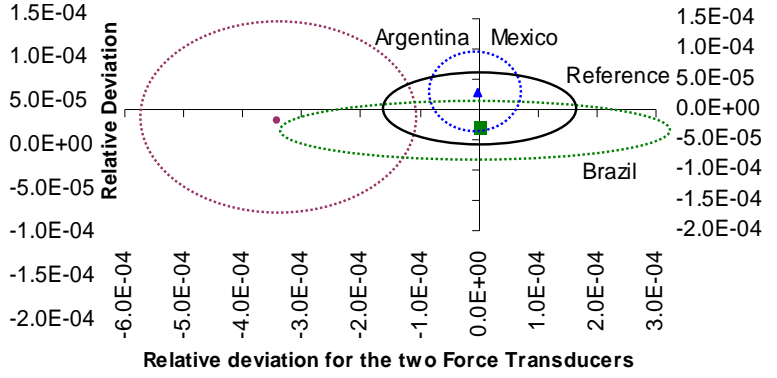
Graph 8. Youden Plot for 5 kN.
